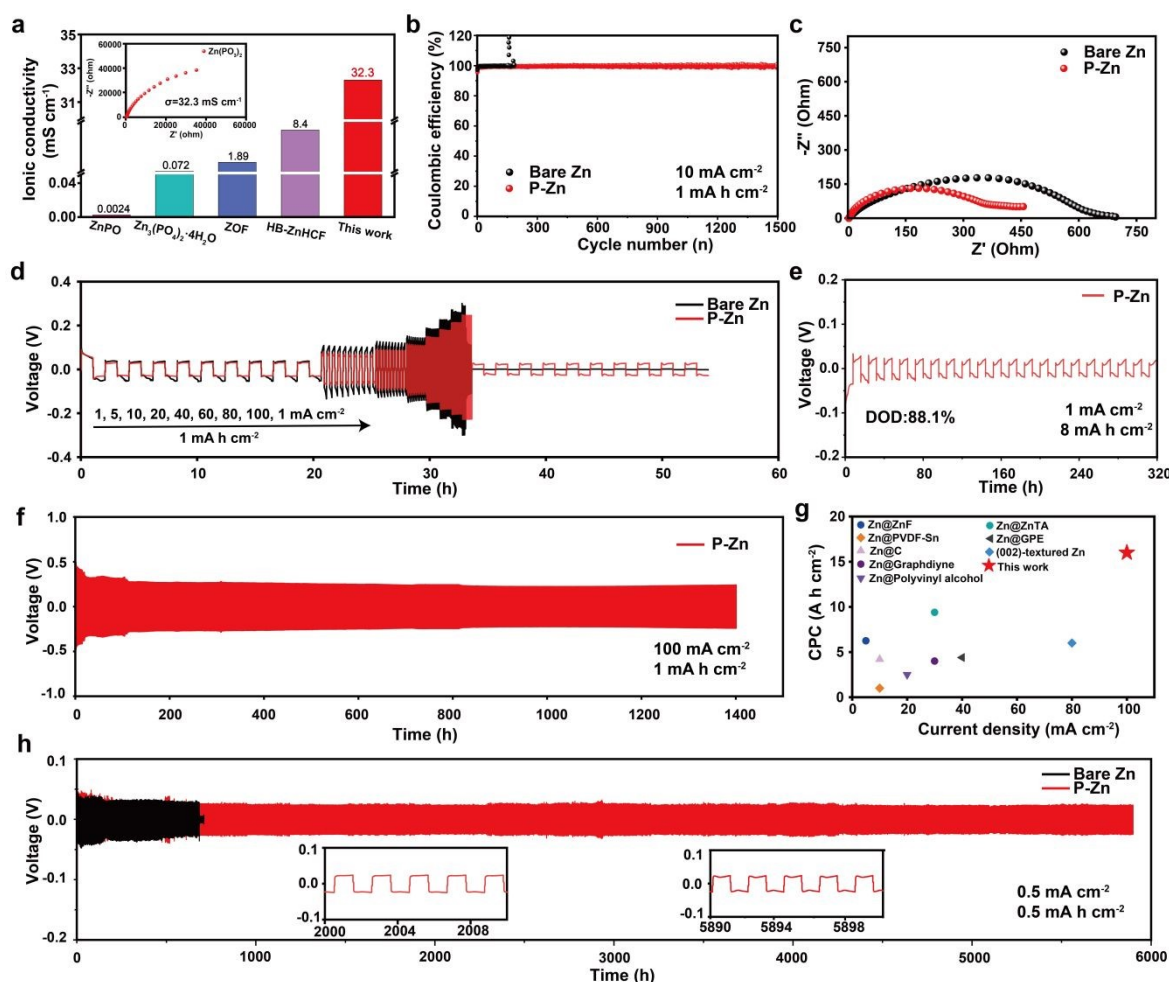
Fig. 2 (a) Comparison of interphase with previous reports in ionic conductivity, inset is the ion conductivity of \text{Zn}(\text{PO}_3)_2 interphase. (b) Coulombic efficiency of bare \text{Zn}||\text{Cu} and \text{P-Zn}||\text{Cu} cells. (c) Electrochemical impedance spectra of symmetric cells after 100 cycles. (d) Rate performances of bare Zn and P-Zn symmetric cells at various current densities. Cycling performance of the symmetric cells using bare Zn and P-Zn at (e) 1 \text{ mA cm}^{-2} and 8 \text{ mA h cm}^{-2} , (f) 100 \text{ mA cm}^{-2} and 1 \text{ mA h cm}^{-2} , and (h) 0.5 \text{ mA cm}^{-2} and 0.5 \text{ mA h cm}^{-2} . (g) Comparison of the symmetrical cells with previous reports in current density and cumulative capacity.
