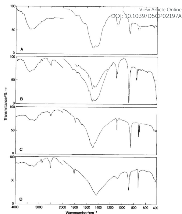
Fig. 2 IR spectra of (A) amorphous \text{CaCO}_3 , (B) vaterite, (C) aragonite, and (D) calcite. Adapted from reference 18 with permission from Scandinavian Society of Chemistry, copyright 1991.
