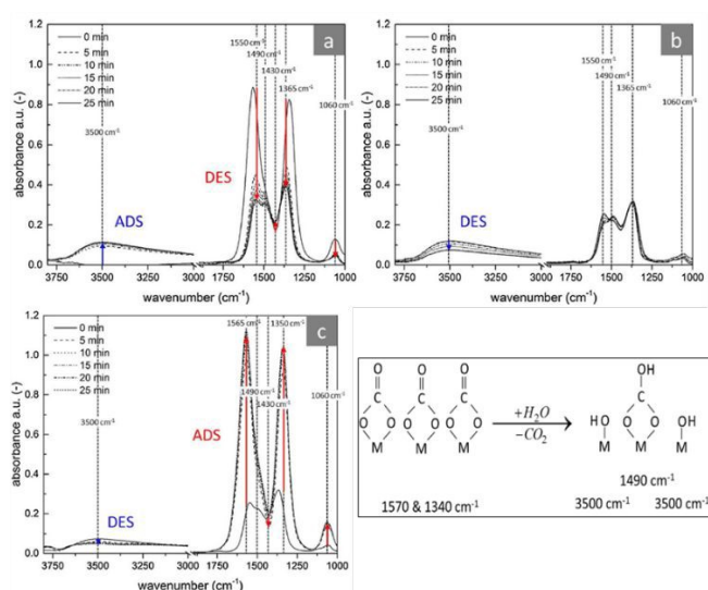
Fig. 15 IR spectra of hydrotalcite after (a) Adsorption of \text{H}_2\text{O} at 400 °C (b) Desorption of \text{H}_2\text{O} at 400 °C with \text{N}_2 (c) Adsorption of \text{CO}_2 at 400 °C after desorption with \text{H}_2\text{O} and \text{N}_2 . The equation shows \text{H}_2\text{O} adsorption and \text{CO}_2 liberation. Adapted from reference 1 with permission from Elsevier B. V., copyright 2018.
