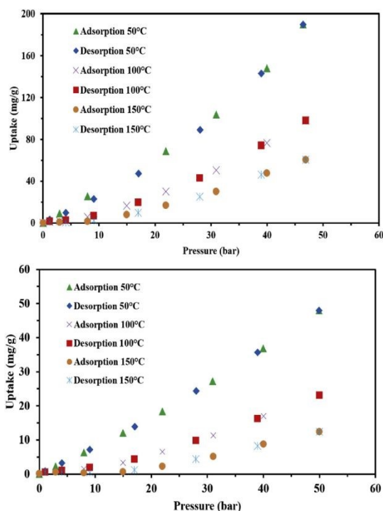
Fig. 18 Evolution with temperature and pressure of the adsorption and desorption of CO 2 (top) and CH 4 (below) on carbonate rocks. Adapted from reference 52 with permission from Elsevier B. V., copyright 2018.
