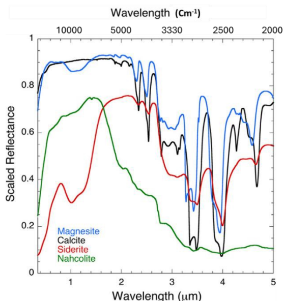
Fig. 4 NIR reflectance spectra (at 2000-28571 \text{cm}^{-1} ) for anhydrous carbonates: calcite, magnesite, siderite, and nahcolite. Adapted from reference 21 with permission from Elsevier B. V., copyright 2015.
