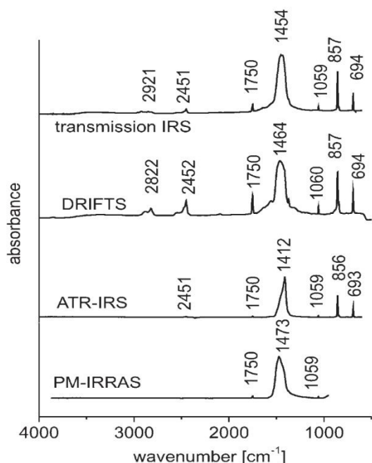
Fig. 1 IR spectra of \text{BaCO}_3 measured by different IR techniques. Adapted from reference 14 with permission from Royal Society of Chemistry, copyright 2008.
