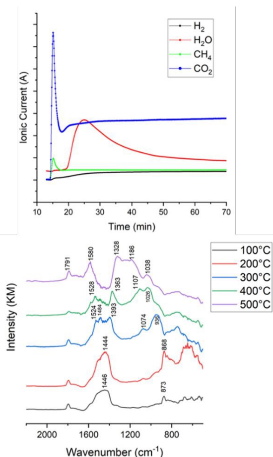
Fig. 12 Operando CO 2 methanation at 400°C on Ni/Dolomite: (Top) Evolution of Mass spectroscopy signal with reaction time. (Bottom) In situ DRIFT spectra as a function of catalyst temperature. Adapted from reference 37 with permission from Elsevier B. V., copyright 2024.
