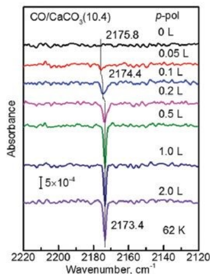
Fig. 11 IRRAS spectra with p-polarized light for CO adsorbed on calcite(10.4) surface at 62 K with increasing exposures (0-2 L). Adapted from reference 34 with permission from Royal Society of Chemistry, copyright 2021.
