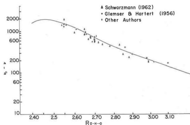
Fig. 9 Relationship between O-H frequency ( \nu ) and O-H...O distance in H-bonds ( R_{\text{O-H}\cdots\text{O}} ); where \nu_0=3756 \text{ cm}^{-1} on the Y-axis. Adapted from reference 28 with permission from Mineralogical Society of America, copyright 1971.
