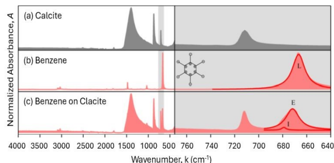
Fig. 16 [Left] IR spectra at 400–4000 \text{cm}^{-1} of (a) calcite, (b) benzene, and (c) benzene on calcite. [Right] Expanded view of 640–770 \text{cm}^{-1} . L: liquid, E: extended adsorption layers, I: first adsorption layer. Adapted from reference 50 with permission from American Chemical Society, copyright 2015.
