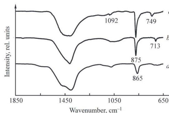
Fig. 5 IR spectra of (a) AOT-ACC, (b) calcite (heating ramp = 10 °C/min), and (c) vaterite (ramp = 1 °C/min). Adapted with permission from reference 23 with permission from Royal Society of Chemistry, copyright 2013.
