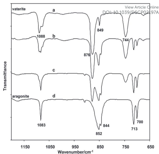
Fig. 8 FTIR spectra (650–1200 \text{cm}^{-1} ) of (a) the vaterite sample, and when it was refluxed in distilled water for (b) 30 min, (c) 60 min, and (d) 75 min. Adapted from reference 27 with permission from American Chemical Society, copyright 2010.
