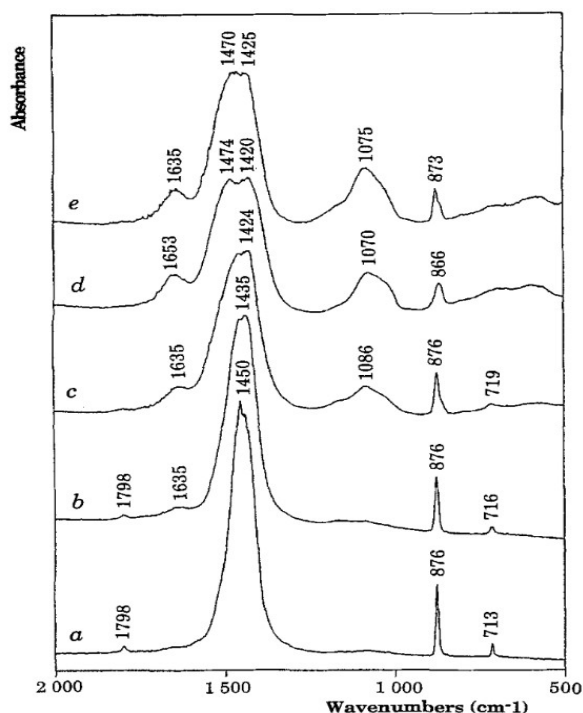
Fig. 7 IR spectra of calcium carbonates from: a) geological calcite; b) separated calcitic cores from the Clathrina spicules; c) intact Clathrina spicules (note the atypical broadening of the calcitic peaks and the additional absorption at 1080 \text{cm}^{-1} ); d) P. pachydermatina spicules; e) synthetic amorphous \text{CaCO}_3 grown in the presence of the macromolecules extracted from the amorphous layer of Clathrina spicules. Adapted from reference 26 with permission from Wiley Online Library, copyright 1996.
