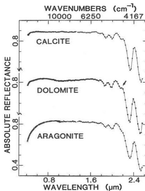
Fig. 3 Vis-NIR reflectance spectra of \text{CaCO}_3 minerals. Adapted from reference 20 with permission from Mineralogical Society of America, copyright 1986.
