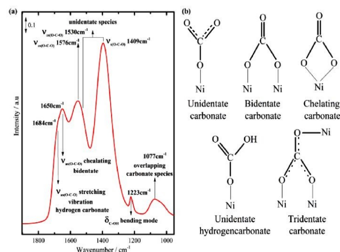
Fig. 13 (a) Infrared spectra of CO 2 adsorbed on Ni-hydrotalcite derived catalyst and (b) Possible species appeared in the CO 2 adsorption experiment. Adapted from reference 38 with permission from Elsevier B. V., copyright 2023.
