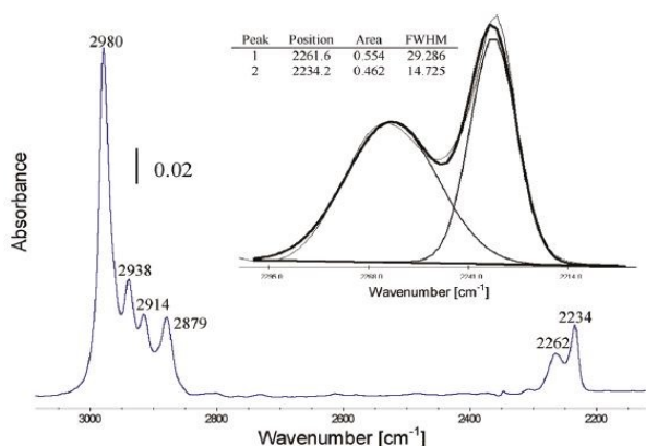
Fig. 17 tert-Butyl cyanide adsorption on carbonated MgO activated at 240 °C. The zoom-in region of 2300–2150 cm -1 . The deconvolution results are shown in the inset. Adapted from reference 4 with permission from American Chemical Society, copyright 2011.
