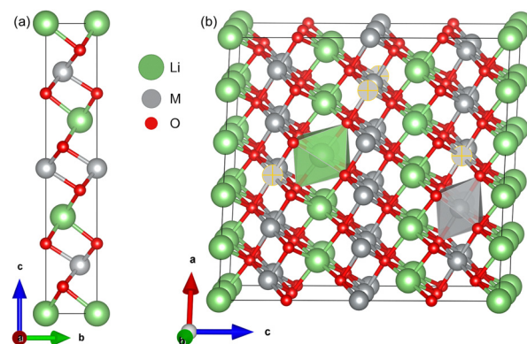
Fig. 1 (a) Unit cell and (b) supercell of LMO, where M = \text{Co or Ni} . Selected atoms show dopant positions in NC91.
