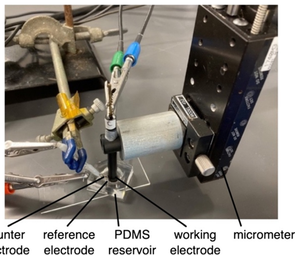
Fig. 2 Experimental setup for the electrochemistry-induced deposition. Adapted with permission from ref. 33. Copyright 2023 American Chemical Society.
