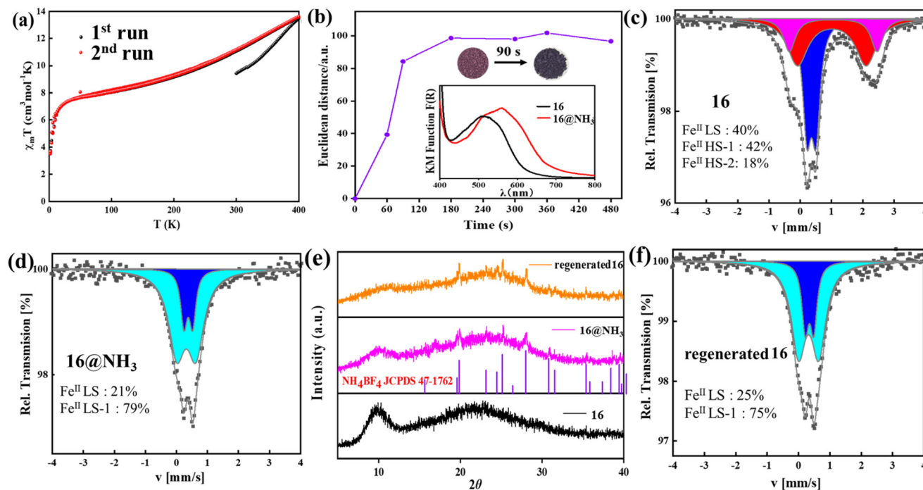
Fig. 15 (a) \chi_m T vs. T plots for microcrystalline cage 16 . (b) Response time curve of 16 to \text{NH}_3(\text{g}) at room temperature. ^{57}\text{Fe} Mössbauer spectrum of 16 (c), 16@NH}_3 (d) and regenerated 16 (f). PXRD patterns of 16 , 16@NH}_3 and regenerated 16 (e). 91
