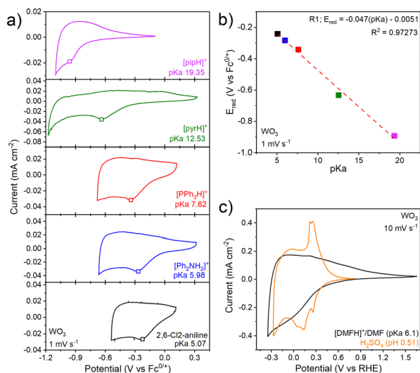
Fig. 2 Electrochemistry of WO_3 in non-aqueous electrolytes containing organic acids ranging in pK_a from 5.07 to 19.35. (a) CVs at 1 mV s^{-1} , (b) pK_a -dependence of the first reduction peak. The red dashed line represents the linear regression fit with a slope of -47 mV pK_a^{-1} unit, (c) CVs at 10 mV s^{-1} in 0.5 M H_2SO_4 and in the non-aqueous electrolyte, 0.1 M [DMFH]⁺/DMF buffer and 0.1 M NBu_4PF_6 in MeCN, both referenced to the RHE potential scale. Open squares in (a) denote the cathodic peak potential, E_{red} , used in (b).
