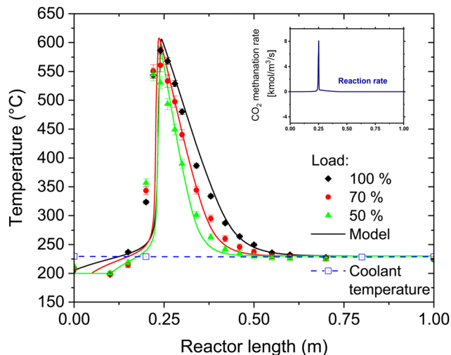
Fig. 5 Temperature profile at different load cases and modelling results (experimental conditions: 8 bar, H 2 :CO 2 = 4.15, CO 2 :CH 4 = 1:1, cooling setpoint = 230 °C, biogas flow = 22 N m 3 h -1 , 80 kg of catalyst in the reactor). The error bars refer to the variation of the temperature in the various experimental runs. In the insert, the calculated methane formation rate (mol L -1 s -1 ) is displayed. The temperature of the coolant remained constant over the entire reactor throughout the experimental tests.
