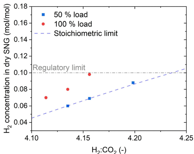
Fig. 4 The effect of stoichiometric ratio on the H 2 concentration in the SNG (experimental conditions: 8 bar, cooling setpoint = 230 °C).
