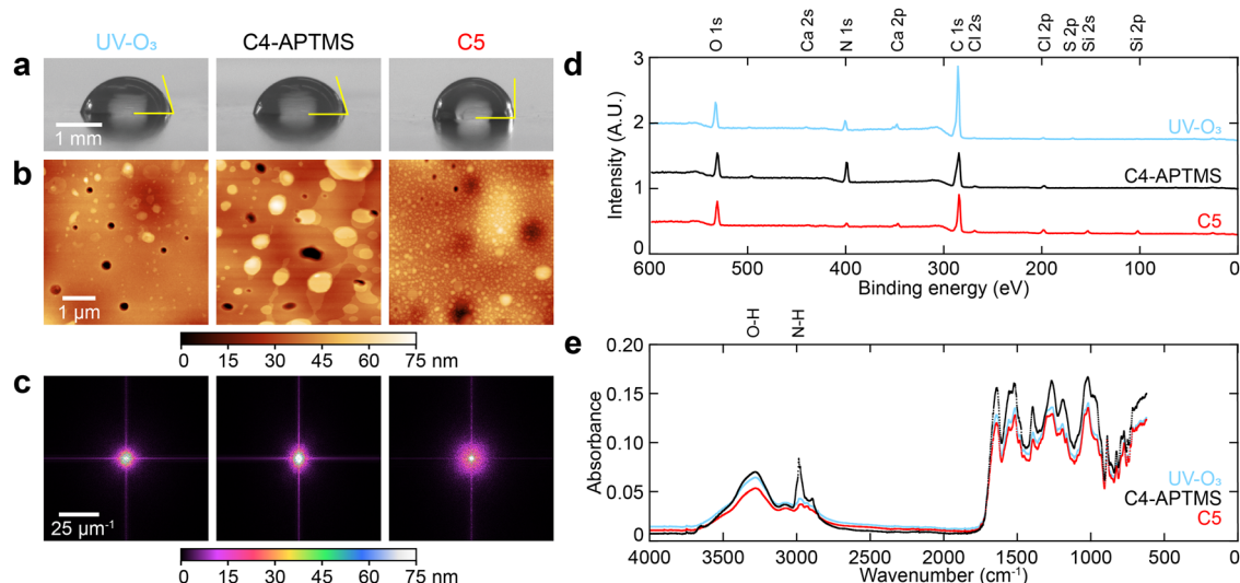
Fig. 2 Materials characterization of card surfaces. (a) Water contact angle of activated surface prior to silane deposition (UV-O 3 ) and the two different surfaces upon successful deposition (C4-APTMS and C5). (b) Height profiles of samples obtained by AFM. (c) FFT representation of AFM surface topography to visualize ordering. (d) Relative intensity of XPS signal (see Table 1), with samples normalized to have equal oxygen peak intensities. (e) Data obtained by FTIR of fresh examples of each sample.
