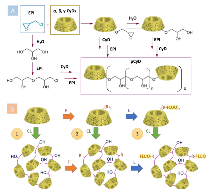
Figure 2: A) General synthetic scheme for the preparation of pCyDs using EPI as CLA; B) synthetic strategies for pCyDs functionalizations (CL= crosslinking, F = functionalization, L = labelling)
