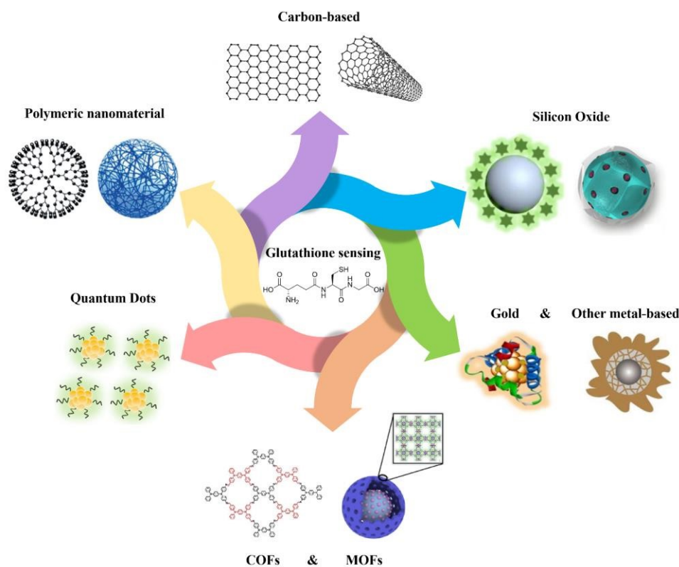
Fig 1. Schematic representation of various kinds of nanomaterials applied for GSH detection. Carbon-based 49 , polymeric nanomaterial 56 , quantum dots 121 , MOFs 95 , COFs 106 , gold 131 , other metal-based 141 , silicon oxide 160,163 schemes are reproduced with the permission of Elsevier, Springer Nature, American Chemical Society, and Royal Society of Chemistry.
