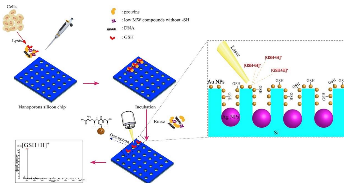
Fig 13. Schematic illustrating the examination of cells. The nanostructured sample spots were loaded with 2 μL of cell lysate, and they were incubated for 10 minutes. The sample spot was cleaned with deionized water and dried in preparation for SALDI-MS analysis after the leftover lysate solution was removed. Reproduced from Ref. 165 with the permission of Elsevier.
