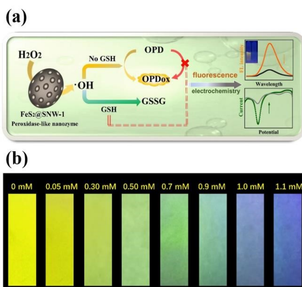
Fig 6. (a) Schematic of a FeS 2 @SNW-1 biosensor for detection of GSH via dual-signal analysis, (b) the fluorescence test paper for GSH detection under UV light of 365 nm. Reproduced from Ref. 109 with the permission of Elsevier.
