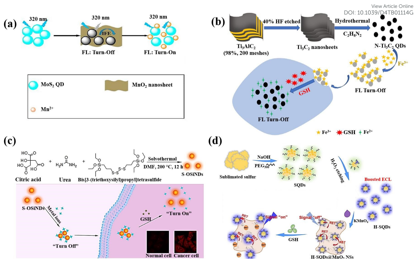
Fig 7. (a) Double-signal MoS 2 QDs/MnO 2 nanoprobe schematic depiction for detection of GSH 117 , (b) N-Ti 3 C 2 QDs/Fe 3+ probe preparation and GSH detection 118 , (c) The production of S-OSiNDs and their use in cancer/normal cell distinction and GSH detection based on the S-OSiNDs' "On-Off-On" fluorescence response feature 120 , (d) H-SQD synthesis and the "off-on" ECL-RET platform design for the detection of GSH 121 reproduced with the permission of Elsevier and American Chemical Society.
