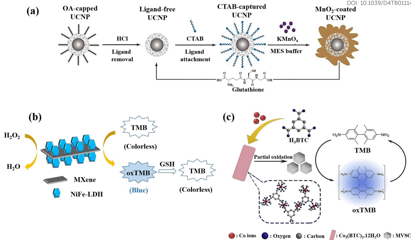
Fig 11. (a) Graphical representation of surface alteration and GSH recognition by employing the \alpha -NaYbF 4 :Tm (1%)@CaF 2 core-satellite UCNP 141 . (b) Colourimetric GSH detection via MXene@NiFe-LDH nanocatalyst 144 . (c) Diagram of preparation of Co 3 (BTC) 2 ·12H 2 O and mixed-valence-state cobalt (MVSC), as well as colourimetric sensor for GSH detection 145 reproduced with the permission of Royal Society of Chemistry, American Chemical Society, and Elsevier.
