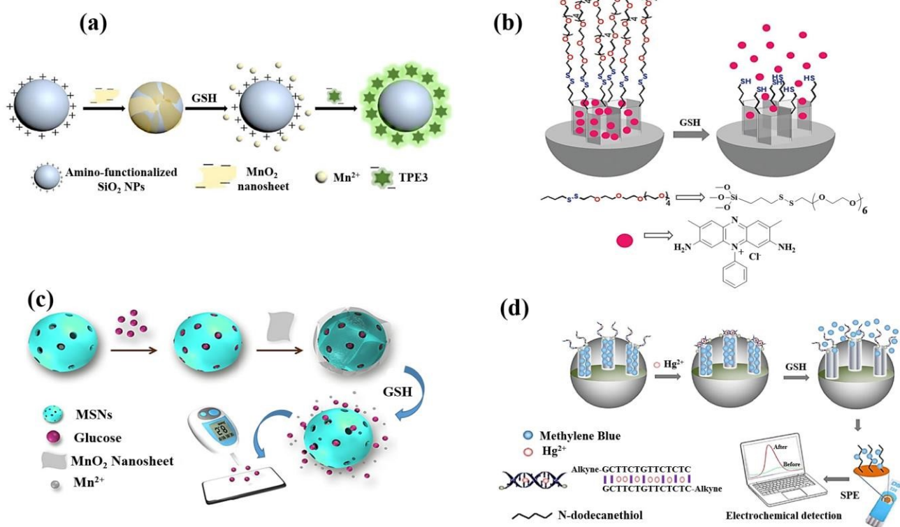
Fig 12. (a) Schematic exhibiting the label-free fluorescence "turn-on" for detecting GSH by employing MnO 2 nanosheets assisted aggregation-induced emission-silica nanoparticles (AIE-SiO 2 ) 160 . (b) Mesoporous silica nanoparticles containing safranin O and coated with oligo(ethylene glycol) chains containing disulfide were employed in the fluorimetry GSH detection 161 . (c) Preparation of the MnO 2 -nanosheet-gated MSNs and the utilization of an external PGM for quantitative GSH detection 163 . (d) Diagram of synthesis of Co 3 (BTC) 2 ·12H 2 O and mixed-valence-state cobalt (MVSC), as well as colourimetric sensor for GSH detection 164 reproduced with the permission of Elsevier, Royal Society of Chemistry, and Springer Nature.
