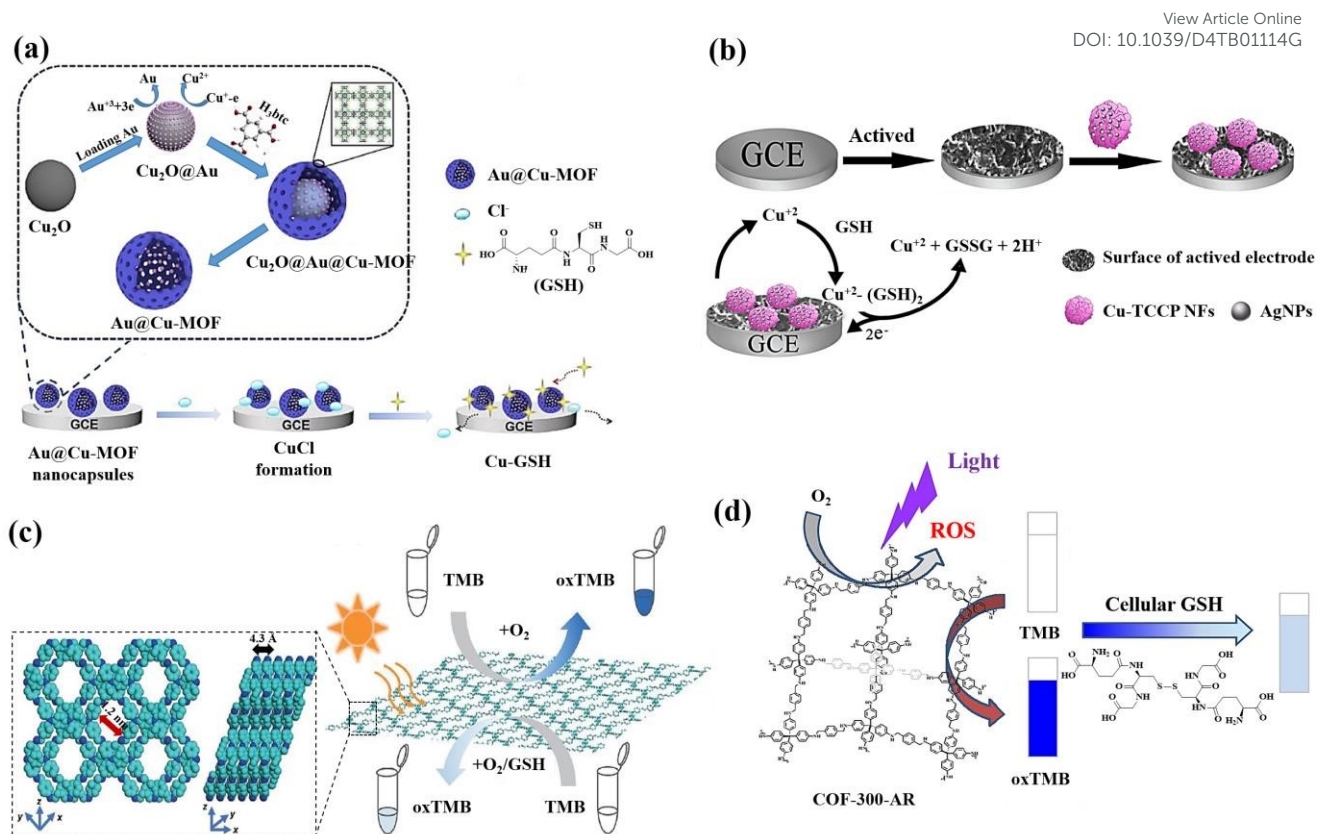
Fig 5. (a) Preparation of Au@Cu-MOF nanocapsules and graphical representation of the sequential steps of the Au@Cu-MOF nanocapsule-modified electrode involving Cl - on electrochemical reactions first, followed by GSH 95 , (b) the fabrication of the electrochemical sensor using Ag/Cu-TCCP nanocomposites and glassy carbon electrodes (GCEs) for the GSH detection based on Possible electrochemical oxidation mechanism of GSH 96 , (c) Top and side view of the energy-minimized models of TTPA-COF and the schematic illustration of GSH detection using TTPA-COF 106 , (d) Schematic illustration of the GSH recognition in cell lysate during visible light irradiation relying on the oxidase-mimicking activity of COF-300-AR 107 reproduced with the permission of Elsevier, American Chemical Society, and Springer Nature.
