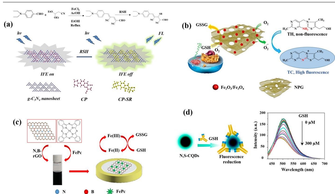
Fig 2. Schematic illustration of GSH detection with carbon-based nanomaterials: (a) the IFE-based fluorescence sensor g-C 3 N 4 nanosheets/CP 51 , (b) the MNPG-based fluorescent assay 54 , (c) the FePc/N,B-rGO nanocomposite 57 , and (d) Graphical example of the of N,S-CQDs fluorescence response to GSH along with the fluorescence spectra of N,S-CQDs combined with different levels GSH 58 reproduced with the permission of Elsevier and American Chemical Society.
