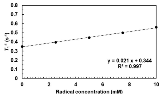
Fig. 5 Plot of T_1 relaxation rates of \text{H}_2\text{O} protons versus the concentration of TTM-PEG3 in water.
