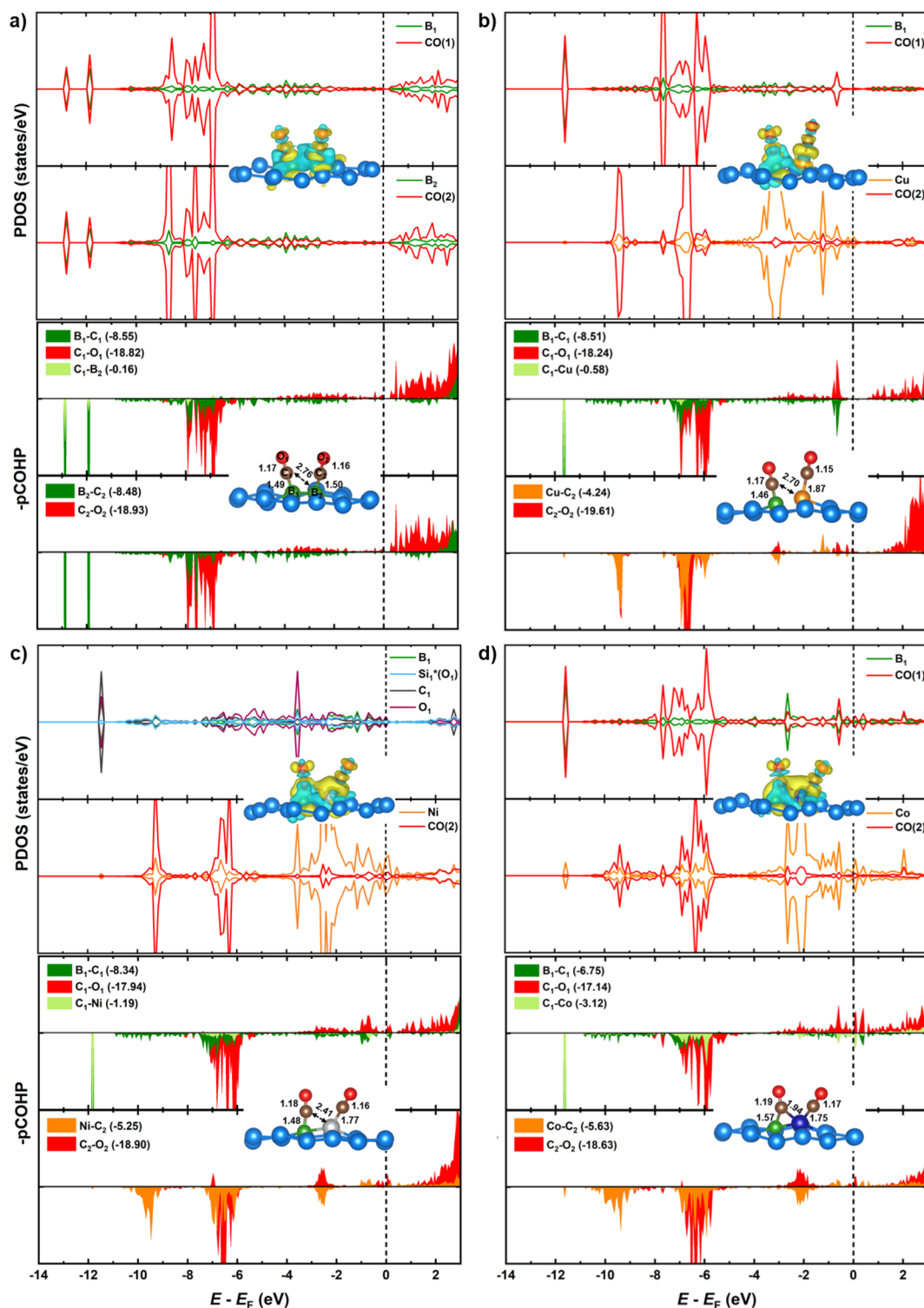
Fig. 7 Partial density of states (PDOS) of dopants and two adsorbed CO^* species (upper panels) on (a) B-B@Si, (b) B-Cu@Si, (c) B-Ni@Si and (d) B-Co@Si. Their corresponding charge density difference are also displayed. The isosurface value is set to 0.0025 \text{ e } \text{\AA}^{-3} , and the yellow (cyan) regions represent charge accumulation (depletion). Projected crystal orbital Hamilton population (pCOHP) of the 2CO^* intermediate. The Fermi level displayed in dashed line is set to zero. Their geometries with bond lengths are also displayed.
