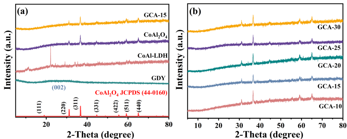
Fig. 2 (a) XRD patterns of \text{GDY} , precursor \text{CoAl-LDHs} , annealed \text{CoAl}_2\text{O}_4 and \text{GCA-15} ; (b) \text{GCA-X} samples.
