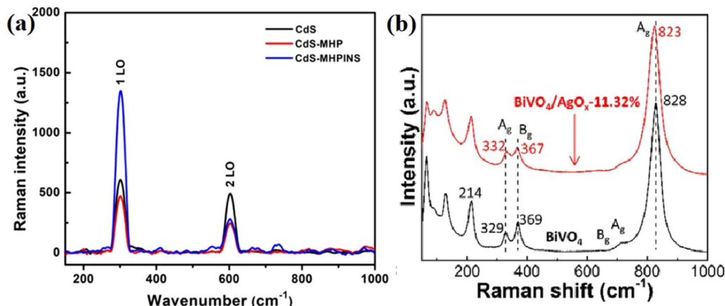
Fig. 13 (a) Raman spectra of the pristine CdS nanowire and heterojunctions of CdS with \text{C}_3\text{N}_5 nanosheets. Reproduced with permission from ref. 89. Copyright 2021, the American Chemical Society. (b) Raman spectra of bare \text{BiVO}_4 and \text{BiVO}_4/\text{AgO}_x -11.32% sample. Reproduced with permission from ref. 42. Copyright 2021, Elsevier.
