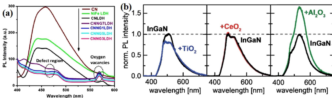
Fig. 14 (a) PL spectra of NiFe LDH, CN, CNLDH and CNNG _x LDH measured at the excitation energy of 380 nm. Reproduced with permission from ref. 78. Copyright 2019, Nature. (b) PL spectra of \text{TiO}_2 -, \text{CeO}_2 - and \text{Al}_2\text{O}_3 -coated InGaN nanowires. Reproduced with permission from ref. 90. Copyright 2018, The Royal Society of Chemistry.
