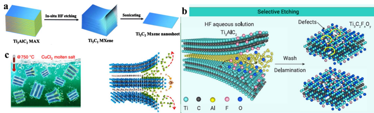
Fig. 3 Synthetic schemes of MXene. (a) \text{Ti}_3\text{C}_2 MXene nanosheets by in situ HF etching, reproduced from ref. 75 with permission from Springer Nature, copyright, 2021. (b) \text{Ti}_3\text{C}_2 MXene nanosheets by HF etching, reproduced from ref. 82 with permission from ScienceDirect, copyright, 2023. (c) Development of a MXene by molten salt, reproduced from ref. 89 with permission from Nature, copyright, 2020.
