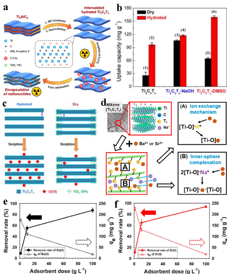
Fig. 22 (a) Synthesis of \text{Ti}_3\text{C}_2\text{T}_x via a hydrated-intercalation approach. (b) Comparative performances obtained for \text{Ti}_3\text{C}_2\text{T}_x , \text{Ti}_3\text{C}_2\text{T}_x\text{-NaOH} , and \text{Ti}_3\text{C}_2\text{T}_x\text{-DMSO} . (c) Sorption of \text{U(VI)} on hydrated and dry MXenes, reproduced from ref. 361 with permission from Royal Society of Chemistry, copyright 2017. (d) Adsorption of \text{Ba/Sr} via MXene. (e) Percentage removal and q_e ( \text{mg g}^{-1} ) of \text{Ba} and (f) percentage removal and q_e ( \text{mg g}^{-1} ) of \text{Sr} by increasing the dose of MXene ( \text{g L}^{-1} ), reproduced from ref. 362 with permission from Elsevier, copyright 2020.
