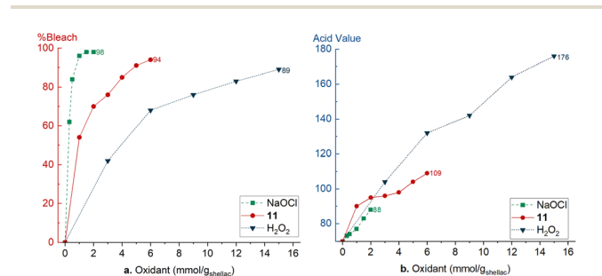
Fig. 2 Comparison of different bleaching methods: NaOCl, \text{H}_2\text{O}_2 and this work with 11 . (a) Bleaching efficiency, (b) acid value.
