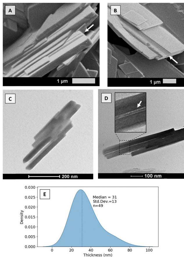
Fig. 2 (A) and (B) Cryogenic scanning electron microscopy of a CNP. The sample was slow-cooled 30% dilution of SSS in OOO (cooled at 1\text{ }^{\circ}\text{C min}^{-1} to 15\text{ }^{\circ}\text{C} ) and visualized after deoiling. (C) and (D) TEM images of CNPs. The inset in (D) presents a magnified view of the lamellar structures. The sample was a deoiled 30% dilution of SSS in OOO, cooled at 10\text{ }^{\circ}\text{C min}^{-1} to 15\text{ }^{\circ}\text{C} . In all cases, white arrows indicate layering structures attributed to lamellar stacking. (E) Kernel density estimators of the thickness of CNPs measured from TEM images ( n = 49 ). Median and standard deviation values are reported in nanometers.
