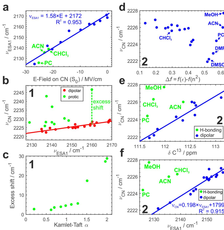
Fig. 4 Electric field vs. hydrogen bonding effects: (a) dependence of the experimental ESA1 band maximum, \nu_{\text{ESA1}} , on the electric field projected onto the C \equiv N bond vector calculated in MD simulations. The electric field on the bond is taken as the average of the fields on the nitrile carbon and nitrogen atoms. Several hydrogen-bonding solvents evidenced by panels (e) and (f) are shown in green. Regression model and R^2 value for the fitted line are shown. (b) Dependence of the ground-state IR absorption maximum, \nu_{\text{CN}} , vs. ESA1 maximum, \nu_{\text{ESA1}} , for compound 1 in aprotic (red) and protic (green) polar solvents. The red solid line is a linear fit to the aprotic data, and the green line is an illustration of the excess shift induced by H-bonding. (c) Excess shift caused by H-bonding in 1 vs. the Kamlet-Taft \alpha parameter quantifying H-bond donating ability of the solvent. (d) IR absorption maximum vs. the Onsager dipolar reorientation polarizability function for 2 . (e) Correlation between \nu_{\text{CN}} and ^{13}\text{C} NMR chemical shift of the nitrile carbon atom in non-H-bonding (blue, linear fit is also shown) and H-bonding (green) media. (f) Same dependence as in (b) for compound 2 . Regression equation and R^2 value for the fitted line are shown.
