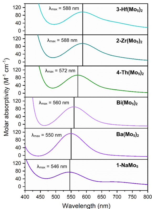
Fig. 4 Electronic absorption spectra of 1-NaMo 5 , 2-Zr(Mo 5 ) 2 , 3-Hf(Mo 5 ) 2 , 4-Th(Mo 5 ) 2 , and the Ba/Bi containing complexes previously reported by Villanneau ( ref. 35). Data collected in MeCN at 21 °C.
