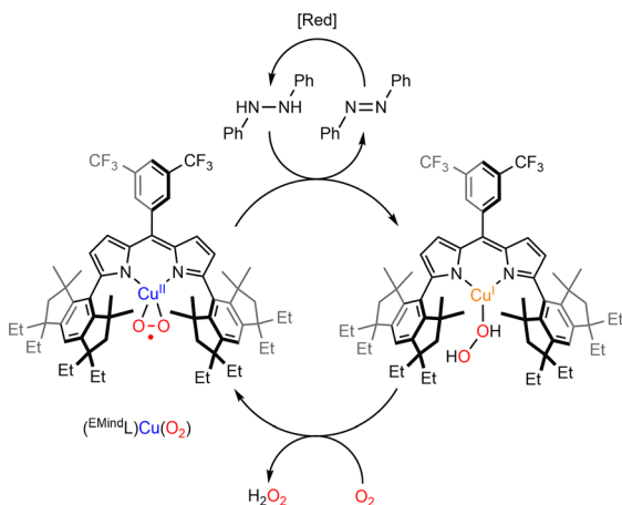
Scheme 7 Reaction of [(^{\text{EMind}}\text{L})\text{Cu}^{\text{II}}(\text{O}_2)] with 1,2-diphenylhydrazine to produce azoarene and [(^{\text{EMind}}\text{L})\text{Cu}^{\text{II}}(\text{H}_2\text{O}_2)] . Adapted from ref. 83.
