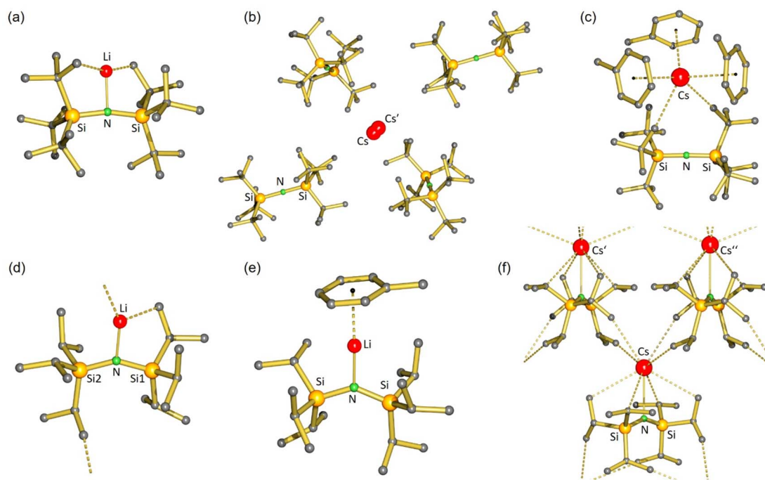
Fig. 2 Crystal structures of (a) (t\text{BuN})\text{Li} (6), (b) (t\text{BuN})\text{Cs} (2), (c) (t\text{BuN})\text{Cs} \cdot (\text{toluene})_3 (2 · toluene 3 ), (d) (i\text{PrN})\text{Li} (9), (e) (i\text{PrN})\text{Li} \cdot (\text{toluene}) (9 · toluene), and (f) (i\text{PrN})\text{Cs} (10). In all cases, H atoms have been omitted for clarity.
