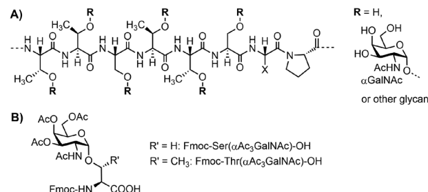
Fig. 1 (A) Tandem repeat motif (TTSTTSP) for MUC5AC. (B) Fmoc-Ser/Thr( \alpha Ac 3 GalNAc)-OH building blocks.
