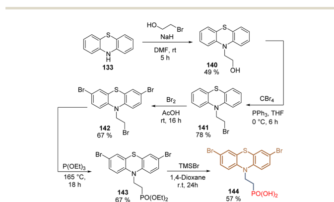
Scheme 18 Synthesis of phenothiazine 144 substituted with electron-withdrawing groups at positions 3 and 7.
