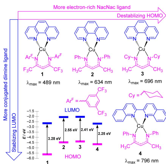
Fig. 2 Summary of heteroleptic Cu(N N )(NacNac R ) complexes and their frontier orbital energy levels. Frontier orbital energies were determined by DFT.
