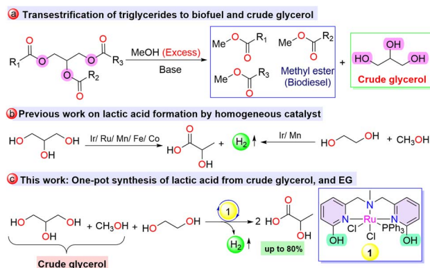
Scheme 1 (a) Crude glycerol generated during the transesterification of triglycerides for bio-diesel production. (b) Homogeneously catalyzed lactic acid formation. (c) Lactic acid formation from a one-pot mixture of crude glycerol and ethylene glycol.
