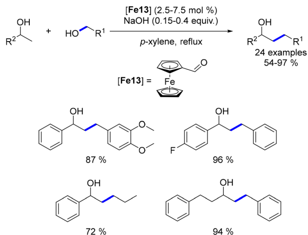
Scheme 73 Iron-catalysed β-alkylation of alcohols.
