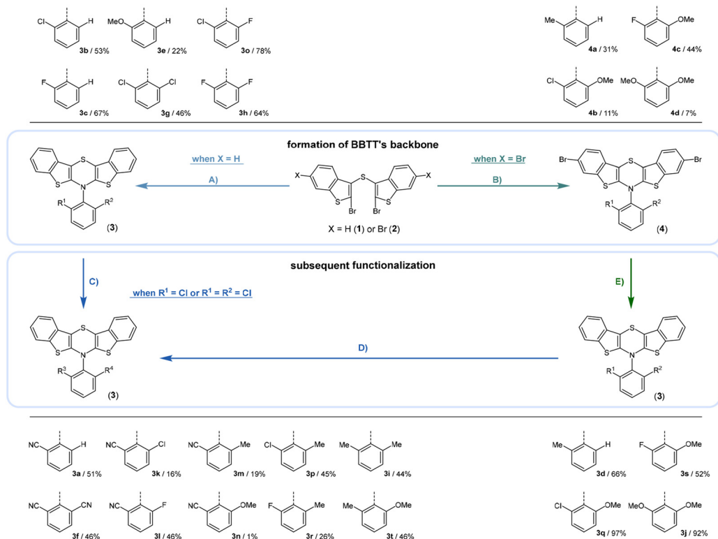
Scheme 1 Modular synthesis of sterically restricted BBTs 3 yielding a functionalization with electron accepting to electron donating substituents in the ortho or ortho,ortho' -position of the N -aryl moiety: (A) ortho ( ortho' )-disubstituted aniline (1.00 equiv.), Pd(dba) 2 (5.00–7.50 mol%), DPPF or XantPhos (10.0–15.0 mol%), NaO t Bu (3.00 equiv.), 110 °C in toluene; (B) ortho ( ortho' )-aniline (1.00 equiv.), Pd(dba) 2 (3.00–5.00 mol%), BINAP (5.00–10.0 mol%), NaO t Bu (3.00 equiv.), 110 °C in toluene; (C) MeMgCl (1.20–2.40 equiv.), PEPPSI-IPr (10.0–15.0 mol%), 60 °C in THF; (D) K 4 [Fe(CN) 6 ]·3H 2 O (0.250–5.00 equiv.), PEPPSI-IPr (5.00–20.0 mol%), Na 2 CO 3 (2.50–5.00 equiv.), 160 °C in DMF; (E) (I) t BuLi (2.40 equiv.), TMEDA (2.40 equiv.), –78 °C in THF and (II) methanol (10.0 equiv.), –78–22 °C in THF.
