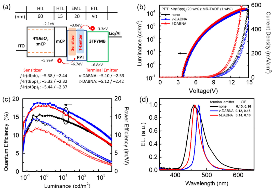
Fig. 5 (a) The energy diagram of all OLED and hyper-OLED devices fabricated in this study, (b) current density–voltage–luminance (J–V–L) characteristics of devices fabricated using f-Ir(tBpp) 3 as a dopant, and devices with Ir(tBpp) 3 as a sensitizer, together with v -DABNA and t -DABNA as terminal emitters, and (c) respective EQE and PE diagrams as a function of luminance, and (d) EL spectra.
