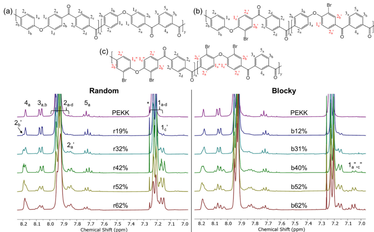
Fig. 5 ^1\text{H} NMR of random (left) and blocky (right) brominated PEKK up to 62 mol% bromination and the corresponding chemical structures of (a) pristine PEKK, (b) monosubstituted BrPEKK, and (c) disubstituted BrPEKK. Assignments are further verified by 2D NMR in the ESI.† Spectra are referenced to \text{CDCl}_3 . The asterisk (*) refers to reference solvent resonance.
