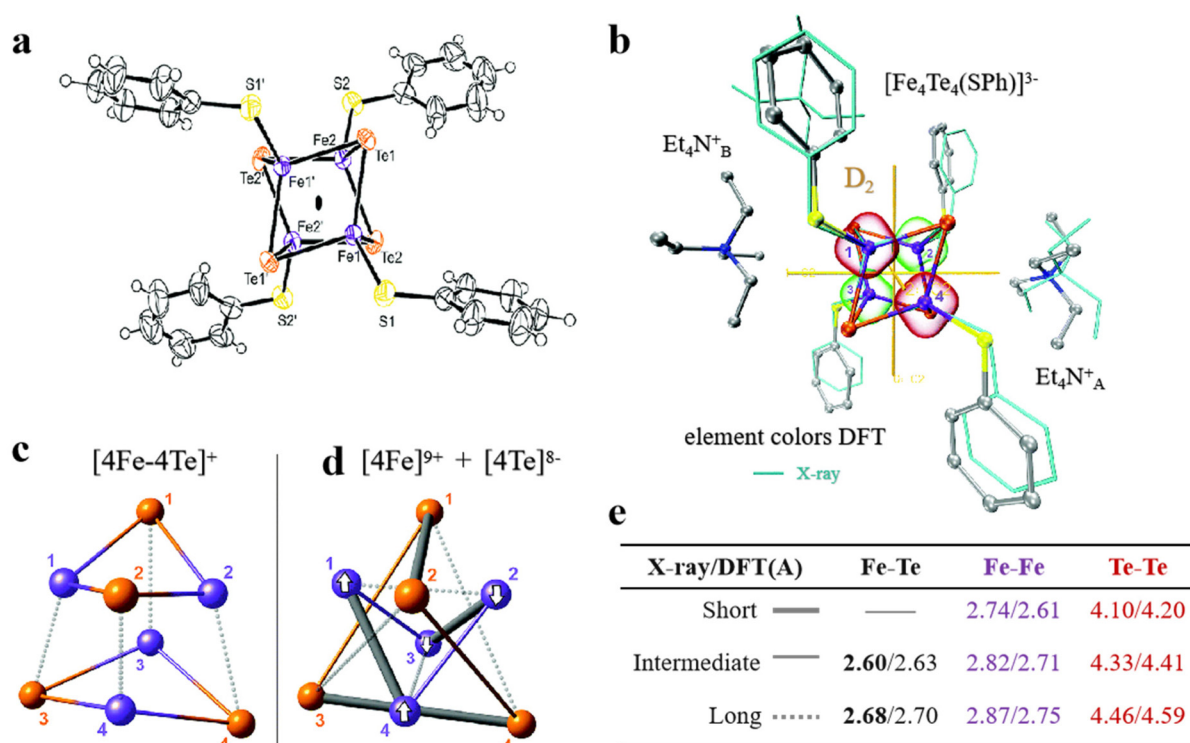
Fig. 9 Artificial Fe-S clusters based on Te element doping. (a) The structure of [Fe 4 Te 4 ] cluster. (b) D 2 -symmetric [Fe 4 Te 4 (SPh)] 3- clusters obtained by X-ray and DFT optimization. (c and d) The bonding interactions and (e) bond length information of [Fe 4 Te 4 ] cluster cores. Reproduced with permission from ref. 98. Copyright 2019, Royal Society of Chemistry.
