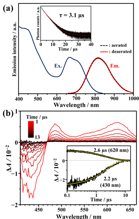
Fig. 2 (a) Excitation (monitored at 850 nm) and emission spectra of AuCu-rod (10 \mu M) in THF. The inset shows the emission decay curve of AuCu-rod in deaerated THF. (b) Time evolution of transient absorption (TA) spectra, measured for AuCu-rod (47 \mu M) in deaerated THF (pump at 670 nm). The inset shows the corresponding kinetic traces of the TA signal at 430 and 620 nm.
