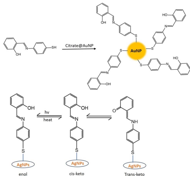
Fig. 9 Mono-iminic Schiff base capping on coinage metal nanoparticle synthesis mechanism.
