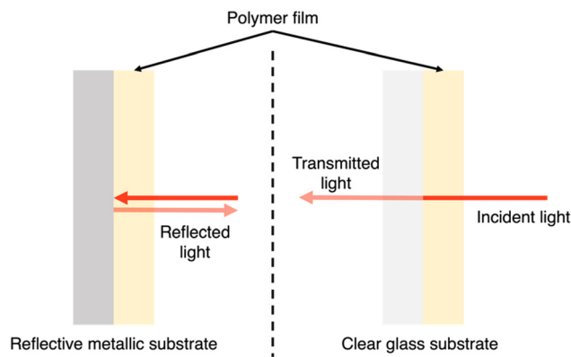
Fig. 23 Schematic representation of the impact a reflective metallic substrate (left) and clear glass substrate (right) has on light transmitted through a polymer film.
