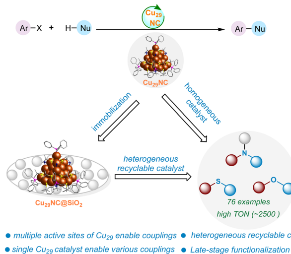
Fig. 1 Catalytic methods for C-heteroatom bond-forming reactions.
