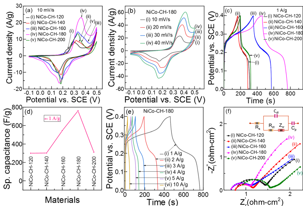
Fig. 4 (a) CV curves of NiCo-CHs synthesized at different temperatures. (b) CV curves of NiCo-CH-180 at different scan rates. (c) GCD plots at 1 \text{ A g}^{-1} and (d) specific capacitance of the NiCo-CHs synthesized at different temperatures. (e) GCD plots of NiCo-CH-180 at different current densities. (f) Nyquist plots of NiCo-CHs synthesized at different temperatures.
