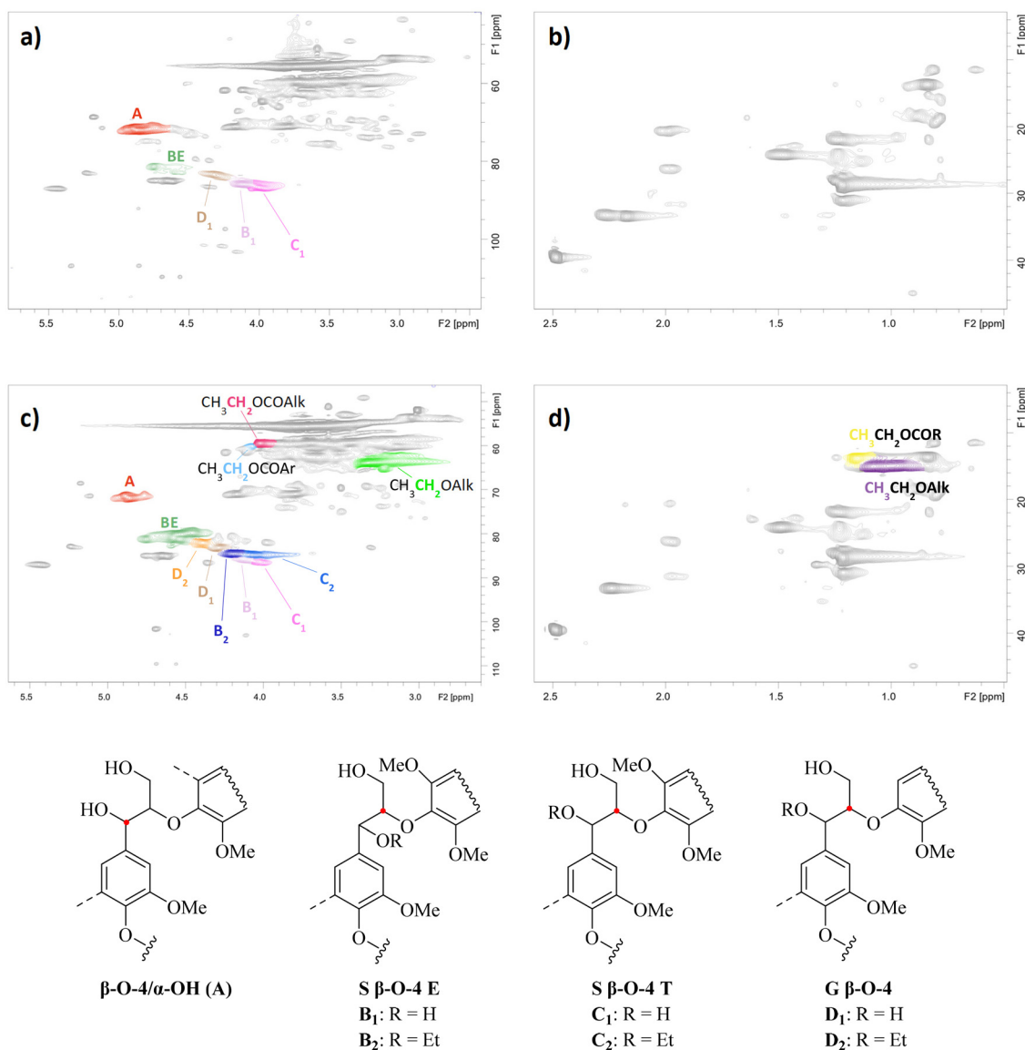
Fig. 3 2D HSQC spectra of ethanol extracted lignin (EEL; a and b) and reactive extracted lignin (REL; c and d). Reaction conditions to produce REL: t = 4 h, [EtOH] = 99%, [H 2 SO 4 ] = 0.15 M, T = \text{reflux} .
