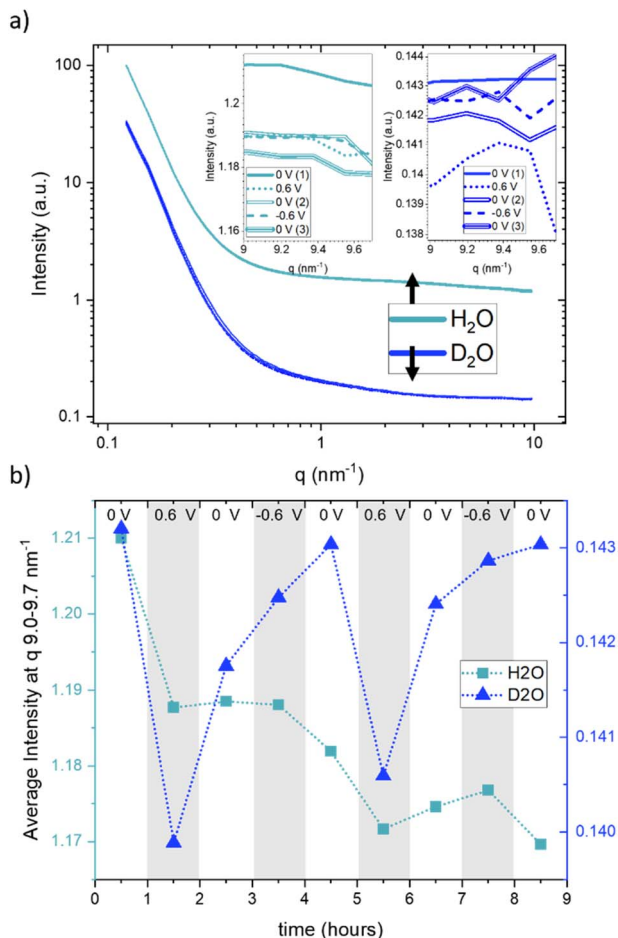
Fig. 3 SANS curves (a) and average SANS intensity in the q -range from 9.0-9.7 \text{ nm}^{-1} (b) for H 2 O (light-blue rectangles) and D 2 O (dark-blue triangles). The insets in (a) show the scattering intensity in the q -range of 9.0-9.7 \text{ nm}^{-1} .
