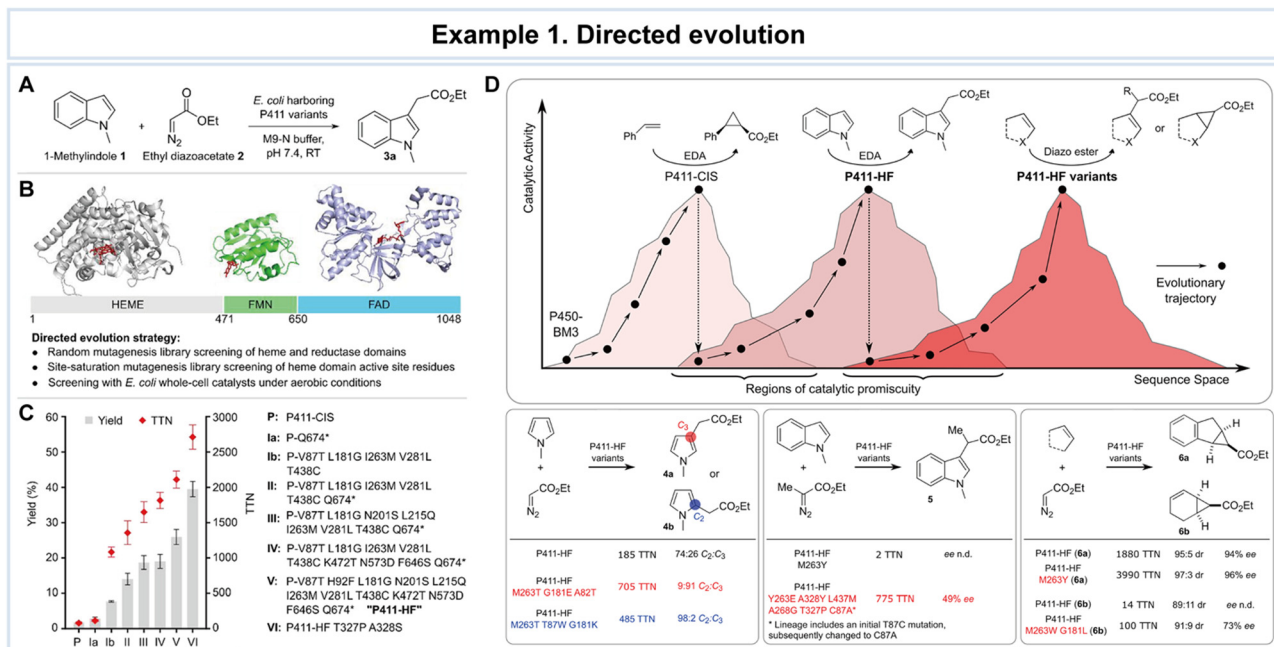
Fig. 6 Representative example of directed evolution for advanced enzyme biocatalysis. Directed evolution of P411-CIS for 1-methylindole C 3 -alkylation. (A) Screening reaction of P411 variants for higher indole alkylation activity. (B) Domain structure of P450-BM3. Individual domain structures with approximate domain boundaries were used to construct the P450-BM3 protein structure. (C) Evolutionary trajectory from P411-CIS to P411-HF T327P A328S. (D) Evolving P411-HF for selective (hetero)cycle functionalization reactions. Schematic representation of the relation between protein sequence and catalytic function. A given enzyme sequence may exhibit additional promiscuous functions that can be optimized by directed evolution. Reproduced with permission from ref. 116. Copyright 2019, American Chemical Society.
