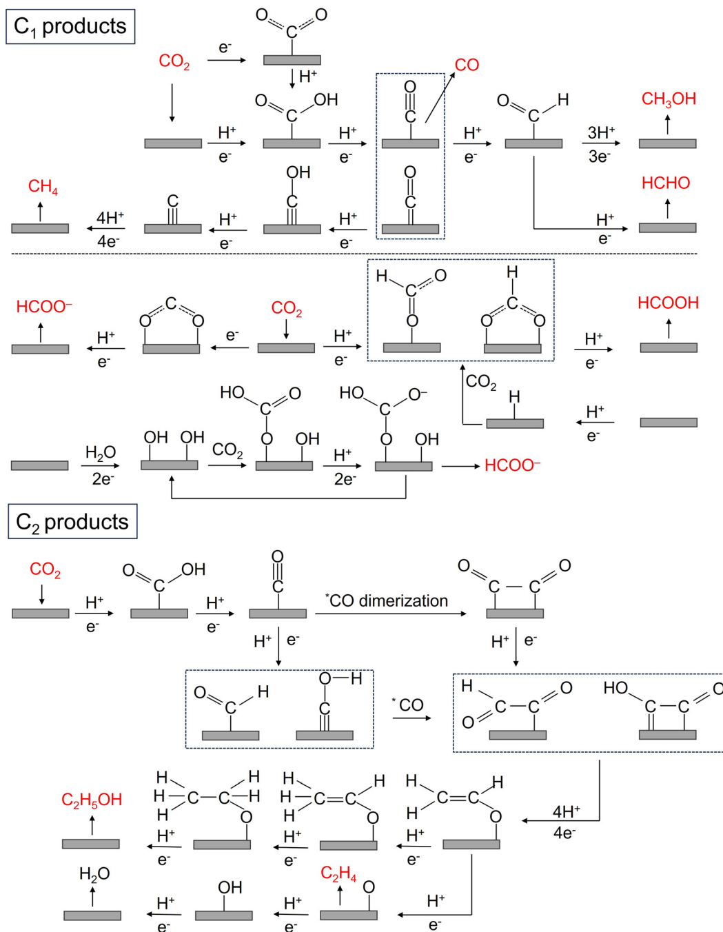
Fig. 3 The possible reaction pathways of \text{C}_1 and \text{C}_2 products in the \text{CO}_2\text{RR} .
