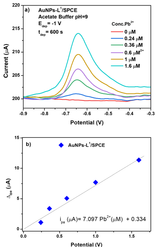
Fig. 10 SWASV voltammograms on (a) AuNPs- L^1 /SPCE in an acetate buffer solution containing a low concentration of Pb(II) ions; conditions: pH = 9.0 , E_{dep} = -1.0 V , and t_{dep} = 600 s . (b) Calibration curve.
