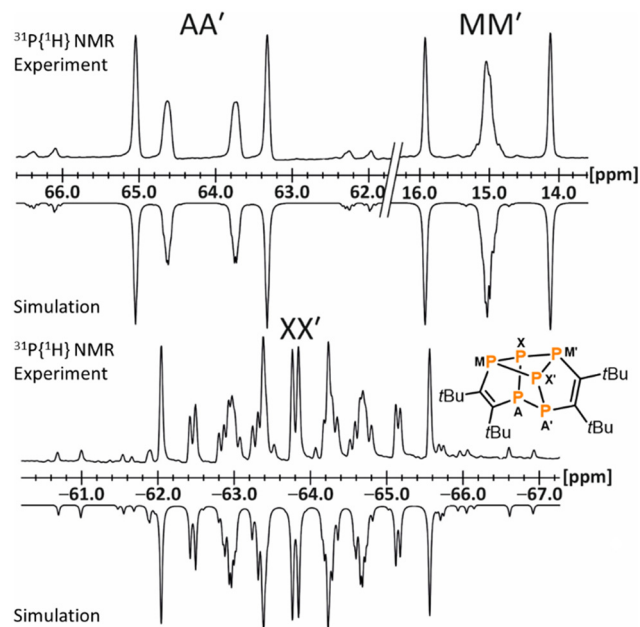
Fig. 6 Sections of the 31 P{ 1 H} NMR spectrum of 13 with nuclei assigned to an AA'MM'XX' spin system; experimental (top); simulation (bottom): δ(P AA' ) = 64.2 ppm, δ(P MM' ) = 15.0 ppm, δ(P XX' ) = -63.8 ppm, 1 J AA' = -261.9 Hz, 1 J AX' = 1 J A'X' = -293.9 Hz, 1 J M'X' = 1 J M'X' = -134.2 Hz, 2 J AM = 2 J A'M' = -3.2 Hz, 2 J A'M = 2 J AM' = 9.9 Hz, 2 J MM' = 24.9 Hz, 2 J AX' = 2 J A'X' = 15.3 Hz, 1 J MX = 1 J M'X' = -157.7 Hz, 2 J XX' = 29.5 Hz.
