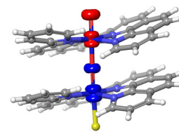
Fig. 2 Spin density distribution of complex 3 [Cl-Fe IV -O-Fe IV =O] 3+ at an isovalue of 0.05 electrons per bohr 3 .
