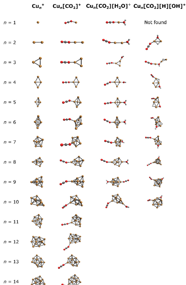
Fig. 3 Lowest energy isomers for \text{Cu}_n^+ , \text{Cu}_n[\text{CO}_2]^+ , \text{Cu}_n[\text{CO}_2][\text{H}_2\text{O}]^+ , and \text{Cu}_n[\text{CO}_2][\text{H}][\text{OH}]^+ in the studied binding modes.
