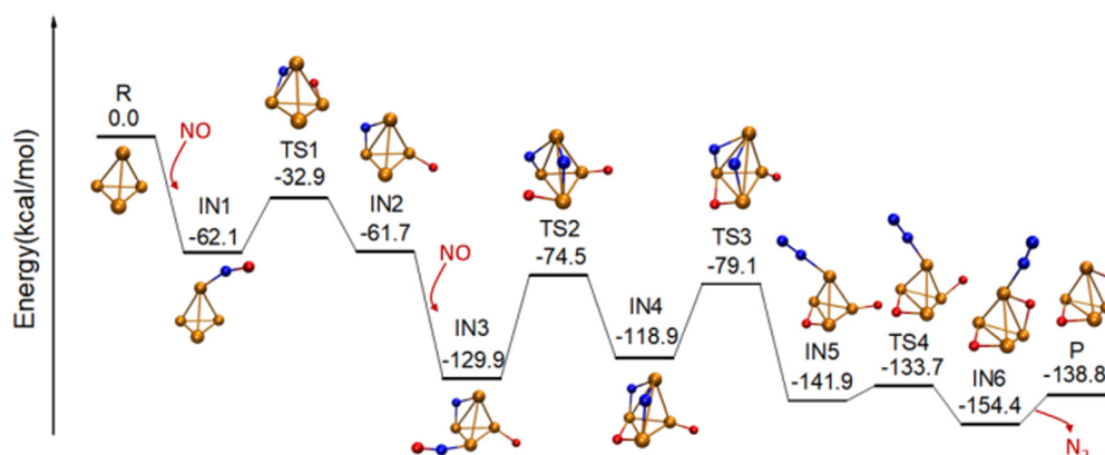
Fig. 2 Reaction pathway of NO reduction on Rh_4^+ calculated at the BPW91/6-31G(d)8SDD level of theory. R stands for reactants, IN for intermediates, TS for transition states, and P for products. All energies are provided relative to the energies of the reactants, i.e., Rh_4^+ and two NO molecules.
