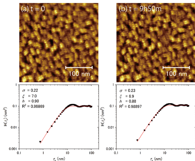
Fig. 7 Topographic images of ASW at 100 K observed at the identical area. Image (b) was obtained 9 h 50 min after the acquisition of image (a). The HHC analysis was applied to the x direction (perpendicular to the deposition direction). No substantial difference was observed between these images and the results of the HHC analysis.
