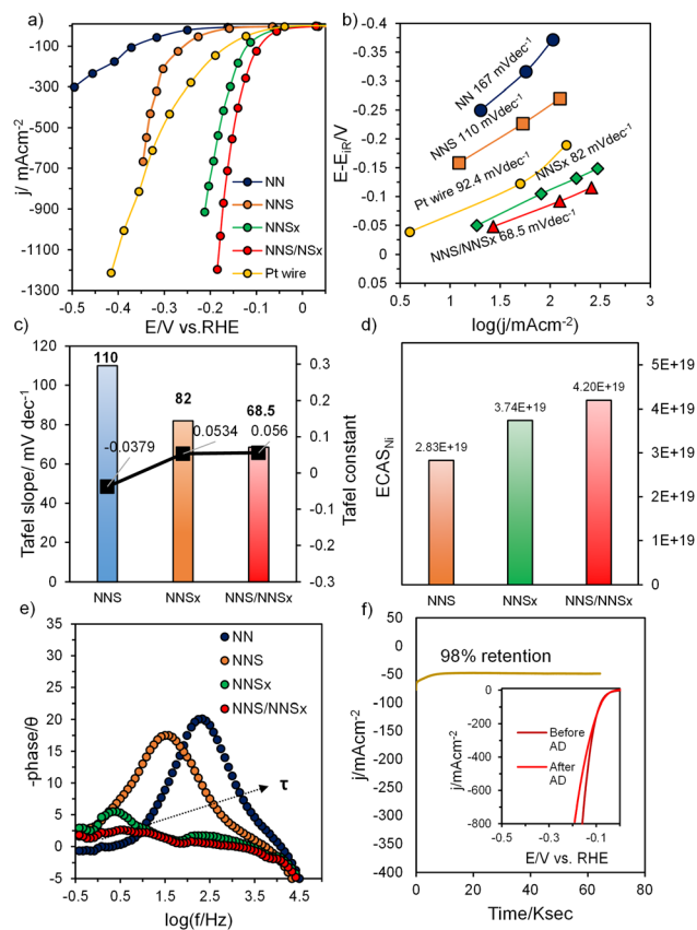
Fig. 4 (a) HER SCV curves with 100% iR compensation; (b) Tafel plots derived from SCV (catalytic turn-over region) for NN, NNS, NNS _x and NNS/NNS _x ; comparative bar diagram showing; (c) Tafel slope and Tafel constant; (d) ECAS _{Ni} for NNS, NNS _x and NNS/NNS _x ; (e) Bode-phase angle plot with time constant and (f) HER stability curve for NNS/NNS _x with the inset showing before and after activity results.
