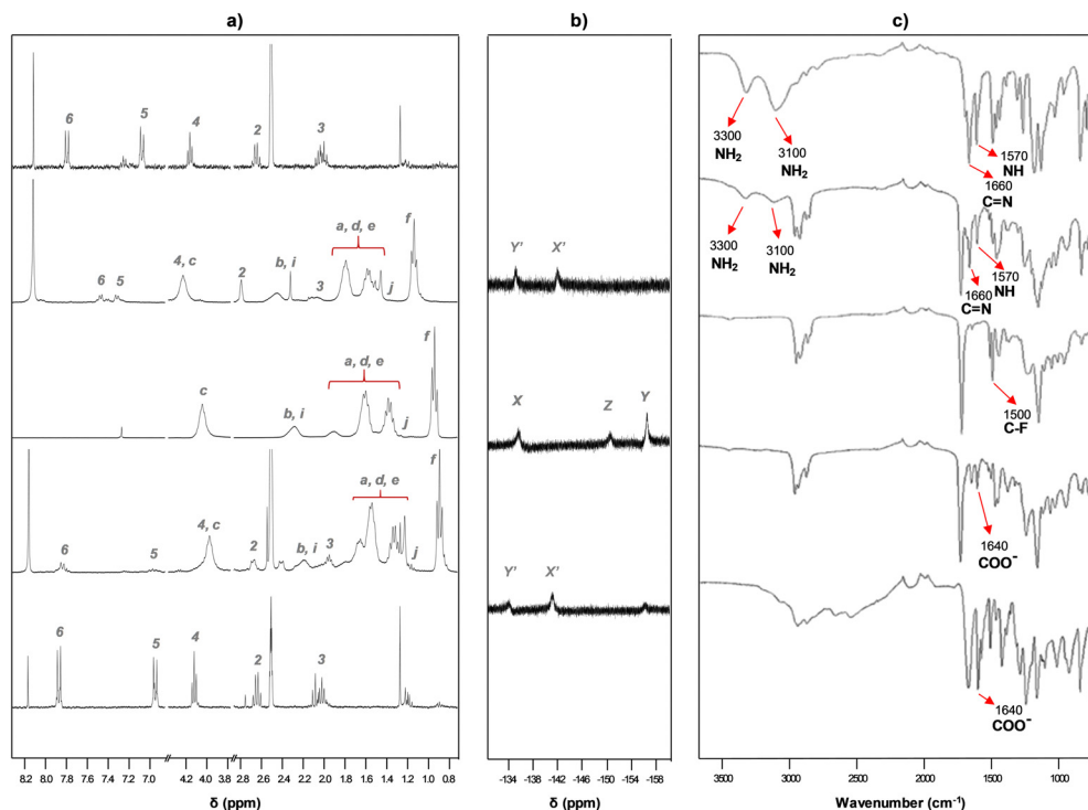
Fig. 2 Representative (a) ^1\text{H} NMR, (b) ^{19}\text{F} NMR and (c) FT-IR spectra of the polymers grafted with A and C units, in comparison with the spectra of the precursor copolymers and the A and C thiols. NMR spectra were recorded in \text{CDCl}_3 : \text{DMSO}-d_6 mixtures.
