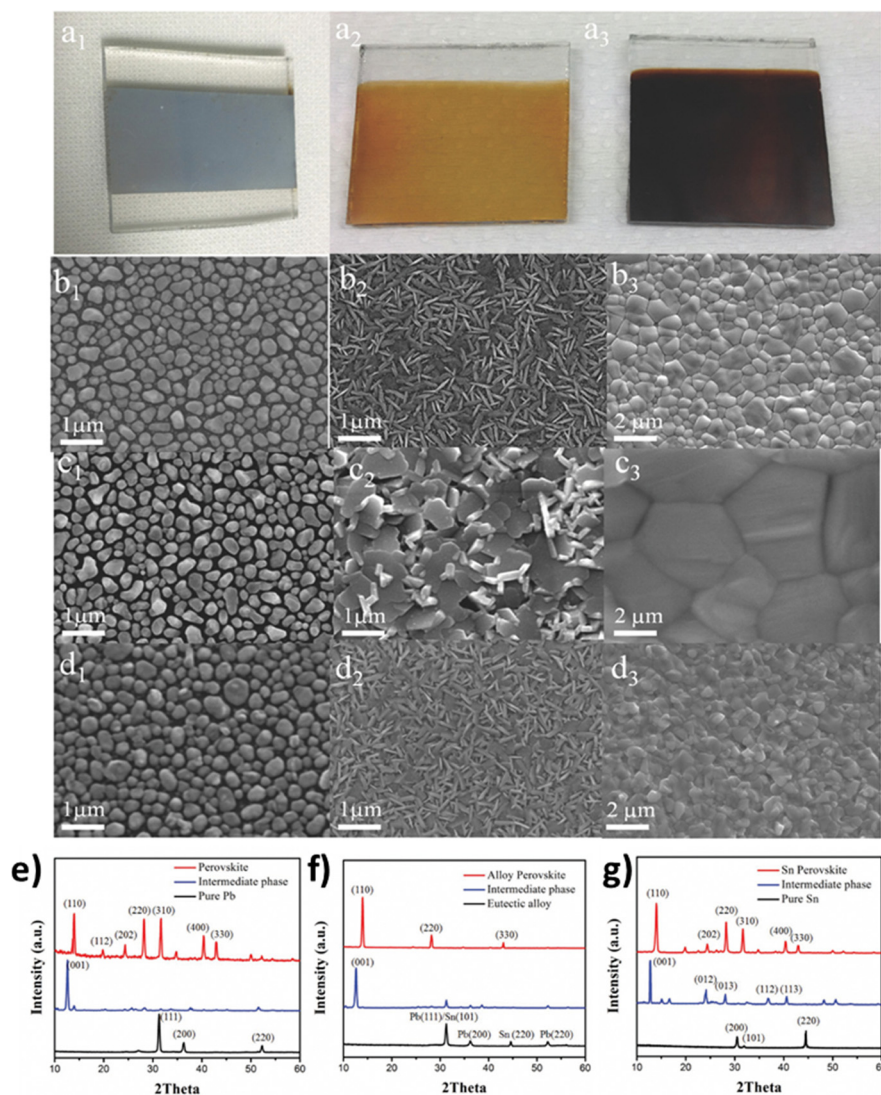
Fig. 9 Photographs of substrates after (a 1 ) deposition of the metal alloy, and after reaction times of (a 2 ) 20 min (intermediate \text{SnI}_2/\text{PbI}_2 phase) and (a 3 ) 40 min (perovskite film). Top-view SEM images of the (b 1 ) Pb metal, (c 1 ) eutectic alloy film, and (d 1 ) Sn metal; and intermediate phases for the (b 2 ) Pb, (c 2 ) eutectic alloy, and (d 2 ) Sn formed after 20 min reaction time; and perovskite films for the (b 3 ) Pb, (c 3 ) eutectic alloy, and (d 3 ) Sn after 40 min reaction time. X-Ray diffraction patterns of metal films, intermediate phases after 20 min reaction, and perovskite films formed by the reaction between the metal precursor and MAI after 40 min, for different metal precursors (e) pure Pb, (f) the eutectic alloy, and (g) pure Sn. Adapted with permission from ref. 118.
