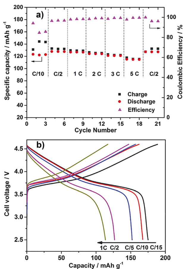
Fig. 10 Electrochemical measurements of 40 wt% \text{Li}_{0.1}\text{Li}_{0.9}\text{b}/\text{PVDF} composites. (a) Specific capacities and coulombic efficiencies of Li/LiFePO 4 cells at different current rates, ranging from C/10 to 5C, 50 ^{\circ}\text{C} . (b) Charge-discharge curves of the Li/LiCo 1/3 Ni 1/3 Mn 1/3 O 2 cell using 40 wt% \text{Li}_{0.1}\text{Li}_{0.9}\text{b}/\text{PVDF} composites (cut-off voltage 2.5–4.6 V), 50 ^{\circ}\text{C} . (Figure partly modified from the original one.) Reprinted from ref. 94 with permission.
