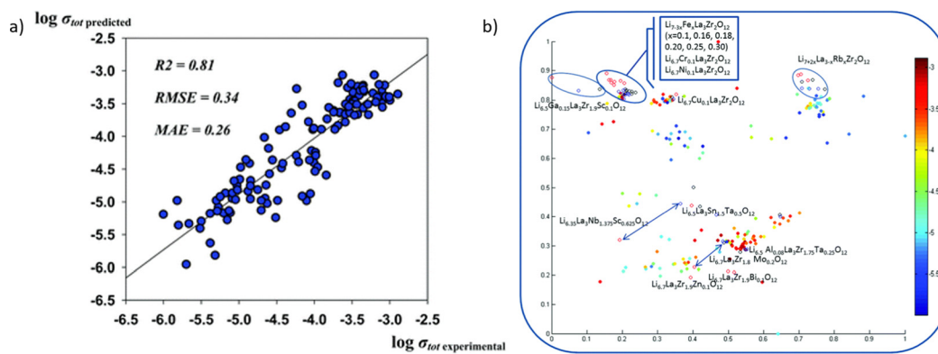
Fig. 13 (a) The prediction accuracy of Li conductivity by machine learning models and (b) the conductivity results categorized using different synthesis methods, and adapt t-stochastic triplet embedding, where experimental results are served as an extra descriptor pool. Reproduced from ref. 261 with permission from the PCCP Owner Societies.
